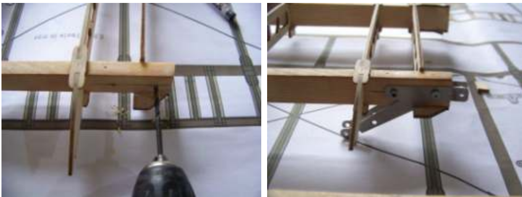
(6) Mark the place of center line and then bore 3mm holes according to the holes of metal parts. And install the metal parts.
